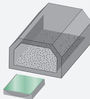
Step 1: Building of a bending mould and laying of the flat glass-blank on the mould
