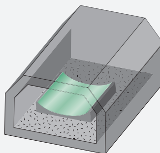
Step 3: The blank sinks into the bending mould
