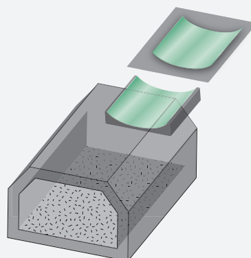
Step 4: ■ In the case of float glass, slow cooling-off (several hours) ■ In the case of heat-strengthened and thermally toughened glass units, fast cooling-off.
